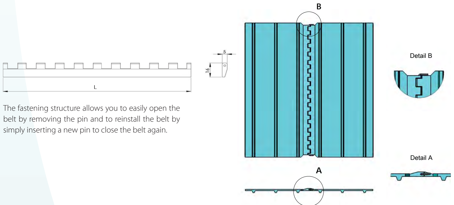
Closing belt with Universal Lace
