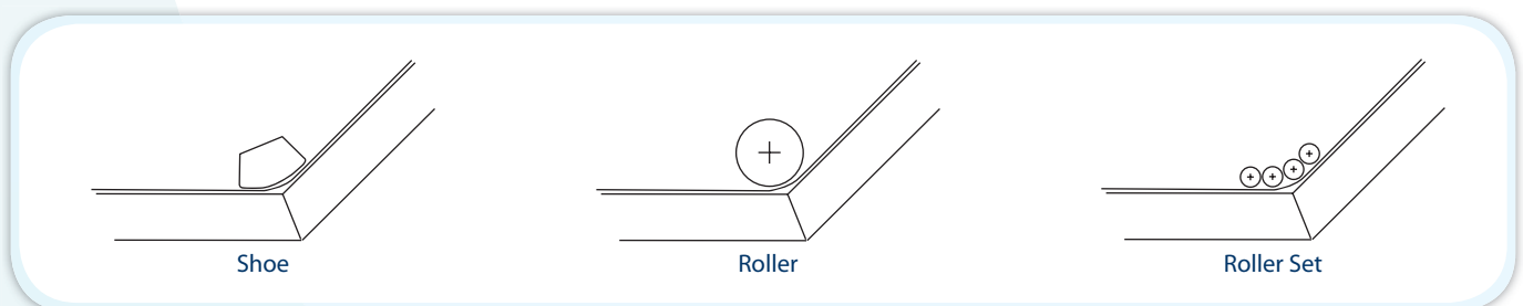
Swan-neck conveyor - transition rollers/ shoe (direction change) options
