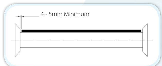
➔ 2. Flanged rollers before the drive side
